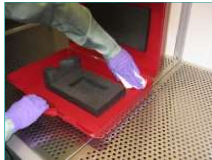
Cleaning of packaging for high performance optics
